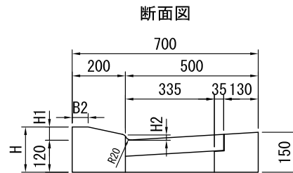
CBL2切下げ型縁塊
