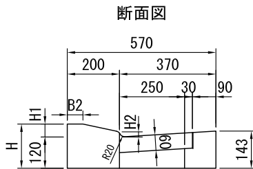
CBL1切下げ型縁塊
